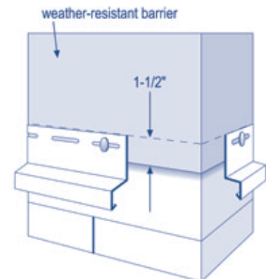
Starter trim at corners
