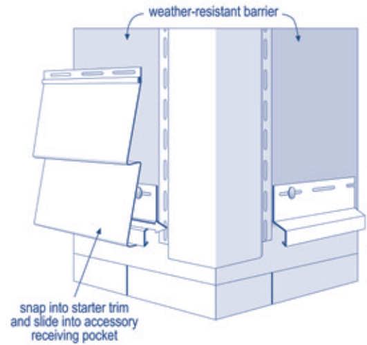
First panel installation
