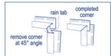
Corner detail B - Mitered corner
