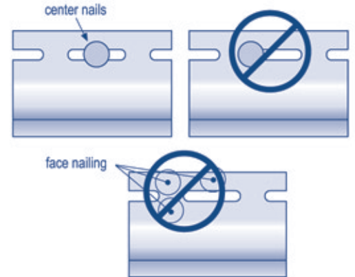
Position of fasteners
