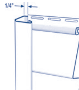
J-channel detail
