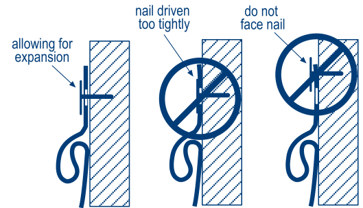
Nailing guidelines
