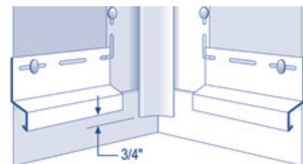
Starter trim and inside corner post
