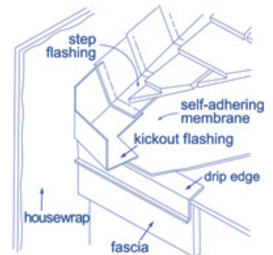
Kickout flashing
