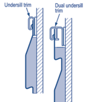
Use of undersill and dual undersill trims when finishing the top of a wall.
