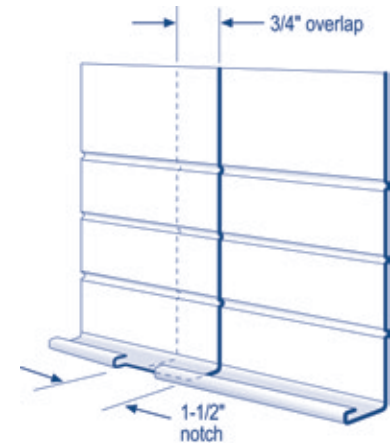
Fascia overlapping
