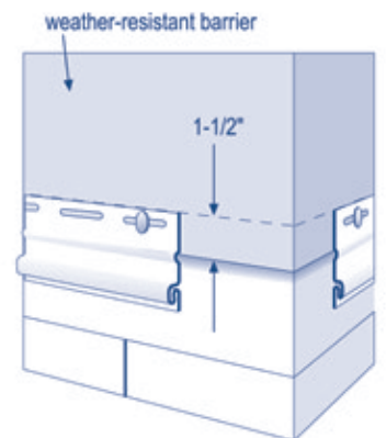
Starter trim at corners
