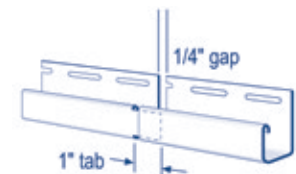
Splicing J-channels
