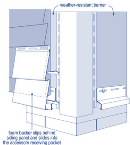
First contoured insulation panel installation
