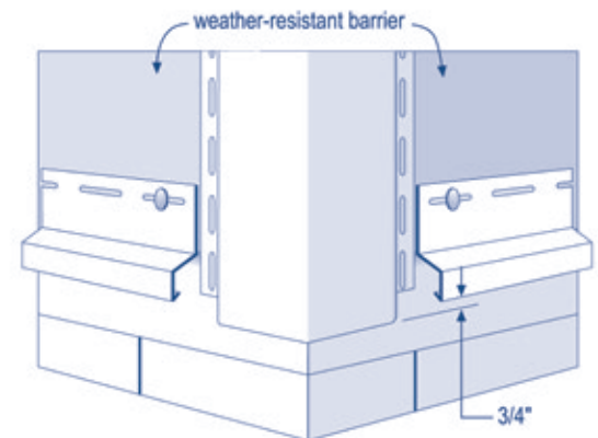
Starter trim and outside corner post
