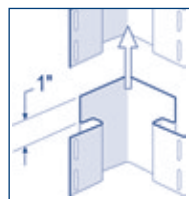
Outside corner splicing detail
