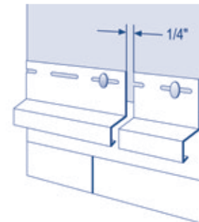
Starter trim installation
