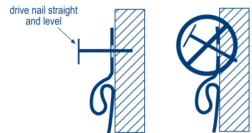
Fasteners detail
