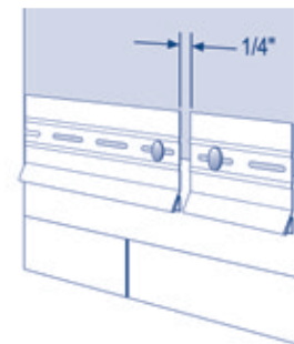
Starter trim installation
