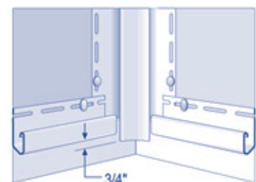
Inside corner detail
