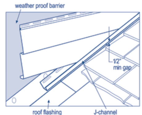
Installation over roof line
