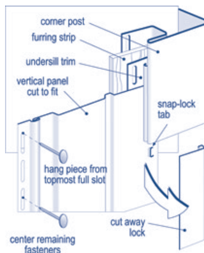
Wall ending detail
